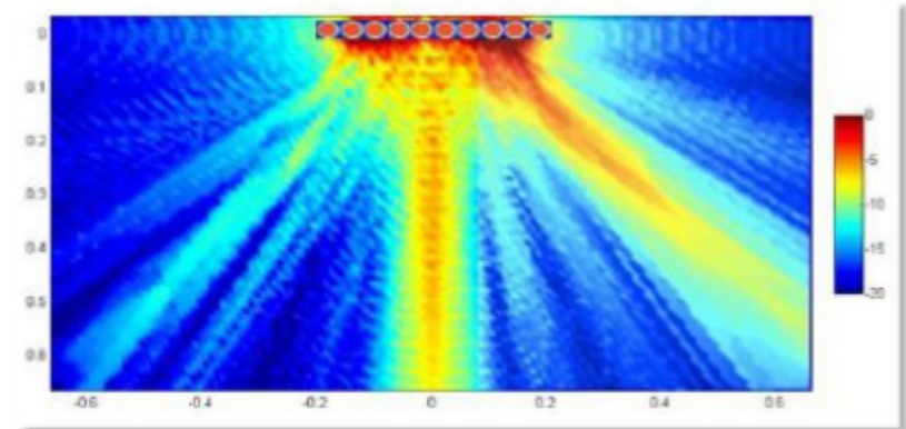
Beamforming with an array of speakers
